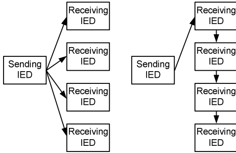
Fig. 5. Hard-wired interdevice signaling.
