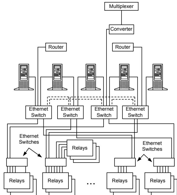
Fig. 1. NamPower network architecture example.
